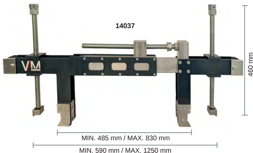
Special CLAMP For CATERPILLAR 980H 25" and 29" rims
