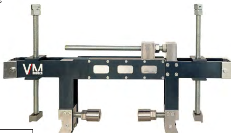
THRUST BUSHING For TRAVEL LIFT MBH 33" and 35" rims
